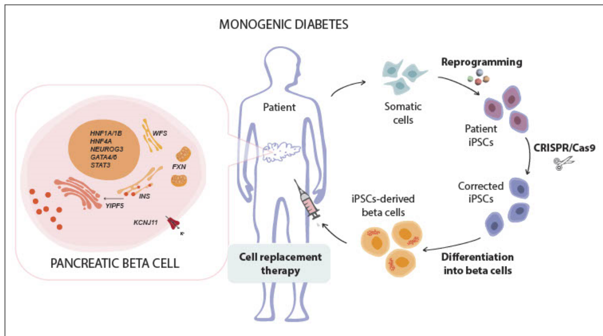
Figure 2. The curative promise of engineered human iPSC-derived beta cells for monogenic diabetes. Monogenic forms of diabetes are caused by mutations in genes critical for beta cell development, function and survival. More specifically, mutations within the HNF4A , HNF1A/1B , NEUROG3 , GATA4/6 , and STAT3 genes impair beta cell development or pancreatic endocrine development and cause maturity-onset diabetes of the young and neonatal diabetes. Mutations within the KCNJ11 gene result in dysfunctional K_{ATP} -channels, which results in impaired insulin secretion. Furthermore, mutations within the YIPF5 gene are responsible for impaired proinsulin trafficking from the endoplasmic reticulum to the Golgi apparatus, giving rise to endoplasmic reticulum stress. Interestingly, other rare disorders, such as Friedreich ataxia and the Wolfram syndrome exist that are accompanied by diabetes. Friedreich ataxia is associated with a reduced expression of the FXN gene, which causes mitochondrial dysfunction, while Wolfram syndrome is characterized by a
